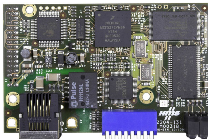
Figure 4-1: EtherNet/IP Module
