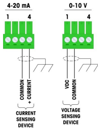
Figure 1-3: Analog Output Kit Wiring Connections
