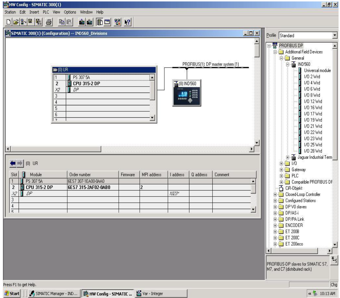
Figure 6-5: Hardware Setup
