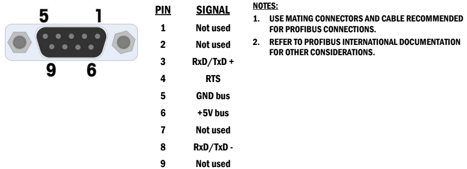
Figure 6-3: PROFIBUS Option Card DB-9 Connector
